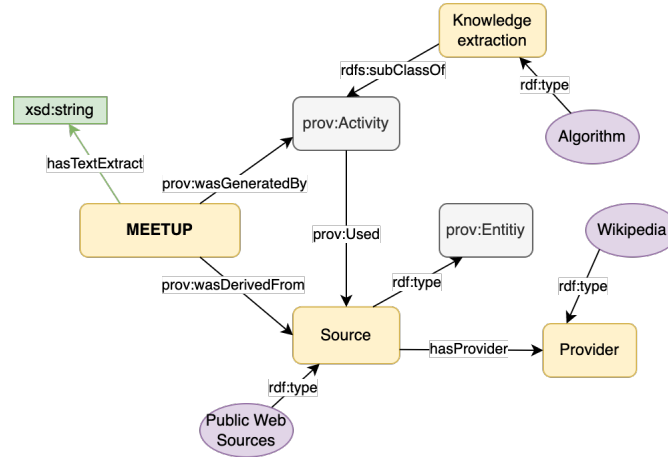
Figure 2: MEETUPS ontology, provenance description
