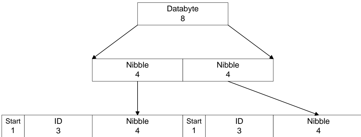
Figure 3.10: Encoding of each byte in the network
