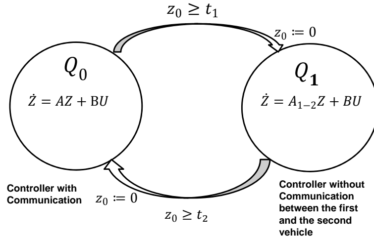
(a) Hybrid Automaton: Example of loss in communication between two vehicles
