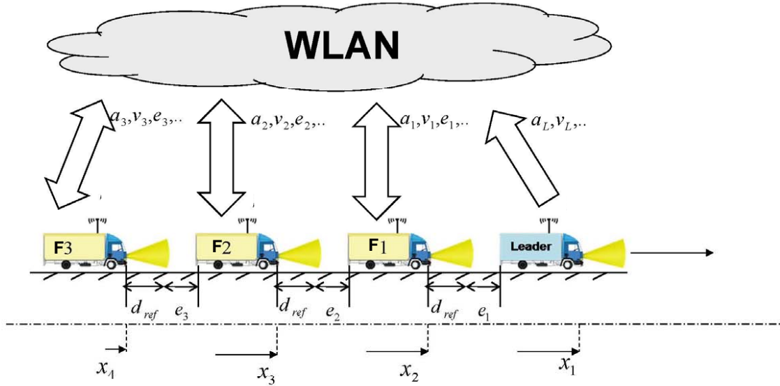
Figure 3.12: The structure of the platoon with notations
