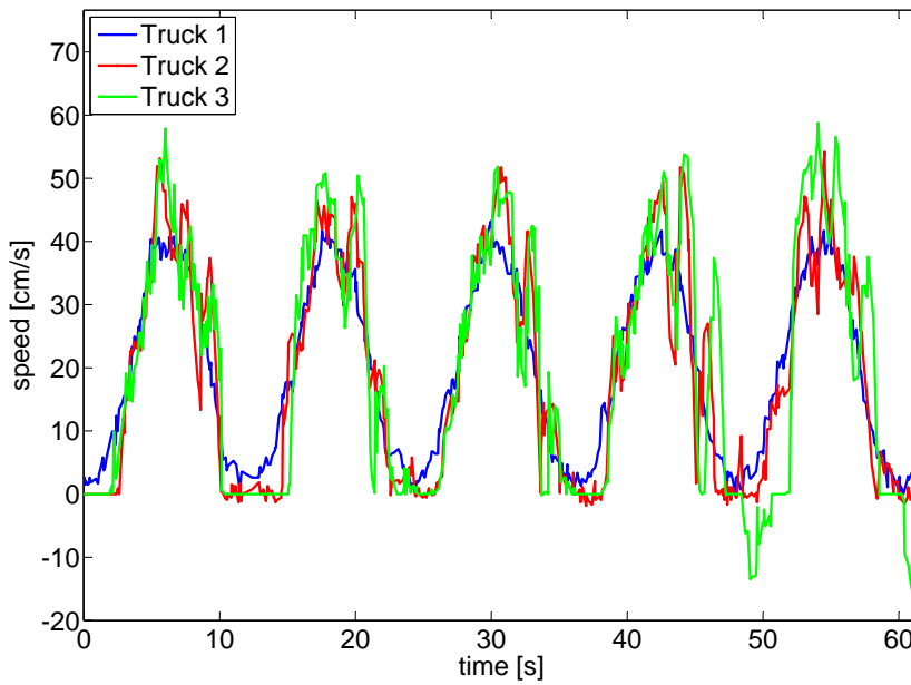
Figure 3.16: Speed vs time: Sinusoidal change of the steering signal
