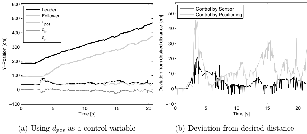
Figure 5.8: Platooning test using the positioning system
