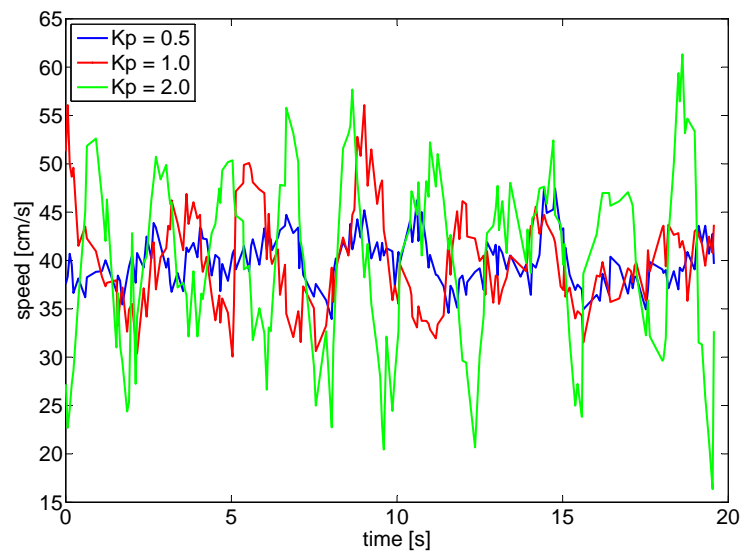
Figure 3.18: Speed VS. time: Different controller modi
