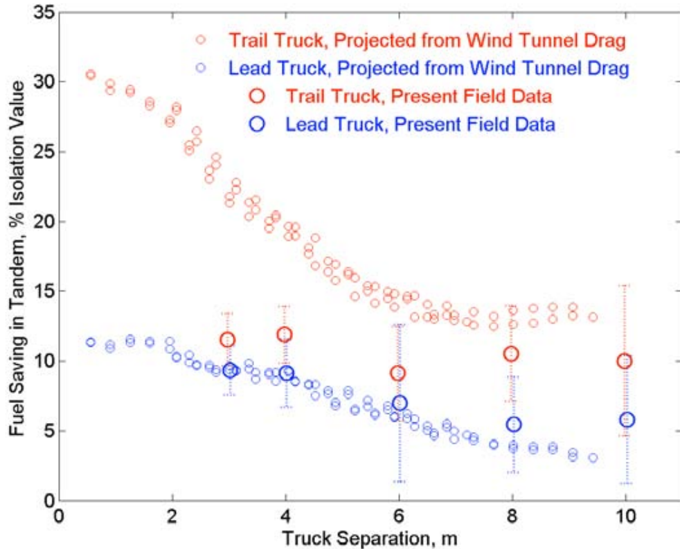
Figure 2.2: Fuel savings for two trucks driving: Comparing the results from field measurements and the wind tunnel tests [22]
