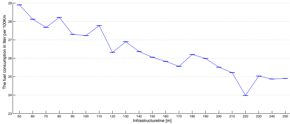
Figure 6.3: Influence of the infrastructure line on fuel consumption
