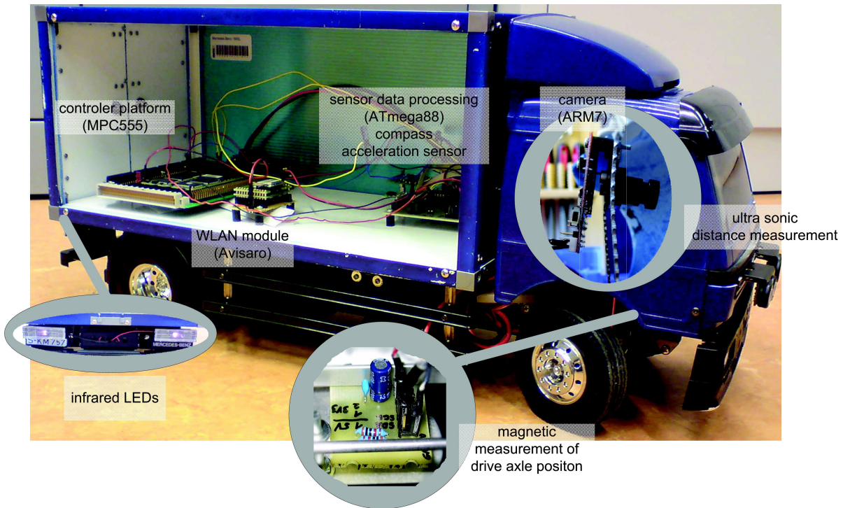
Figure 3.3: The position of hardware modules on each truck
