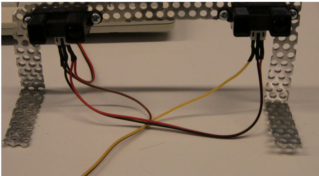
Figure 5.11: Road detectors of the intersection management unit
