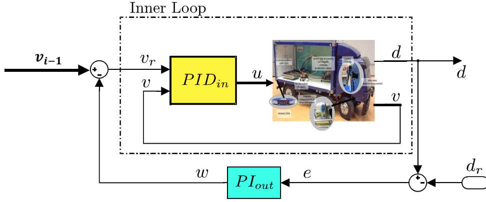
Figure 3.14: Cascade control structure [DCGBM + 10]
