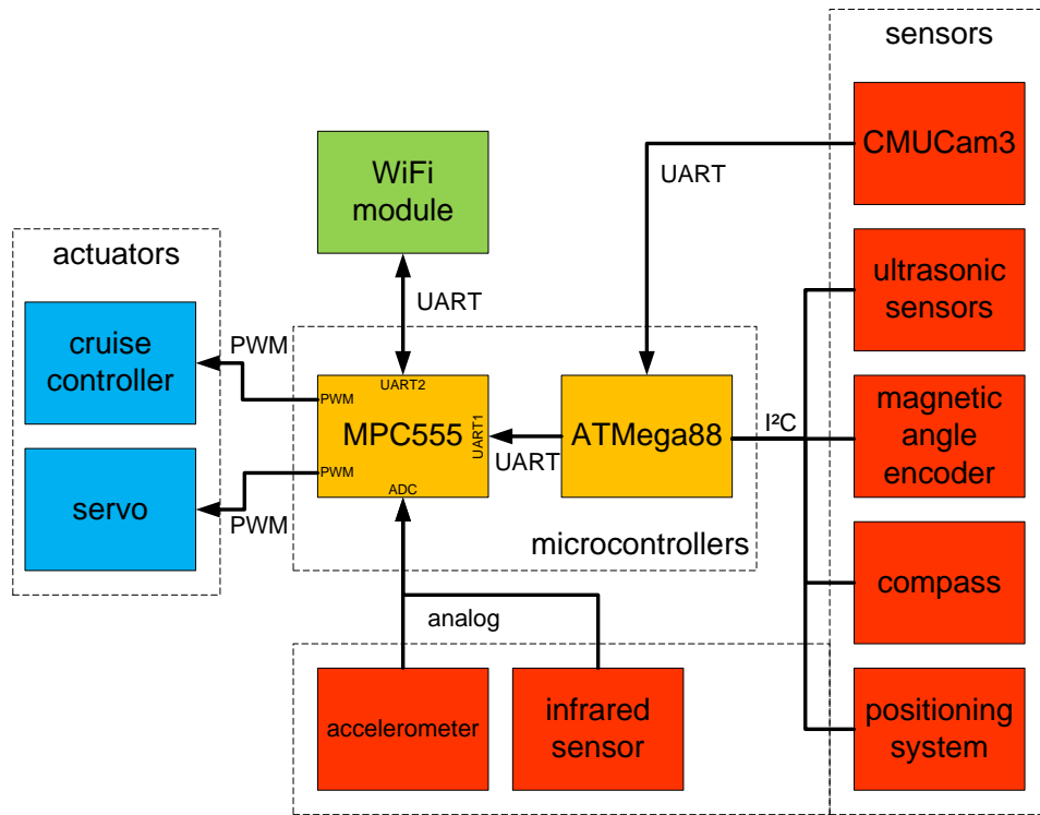
Figure 3.2: Hardware architecture of each truck
