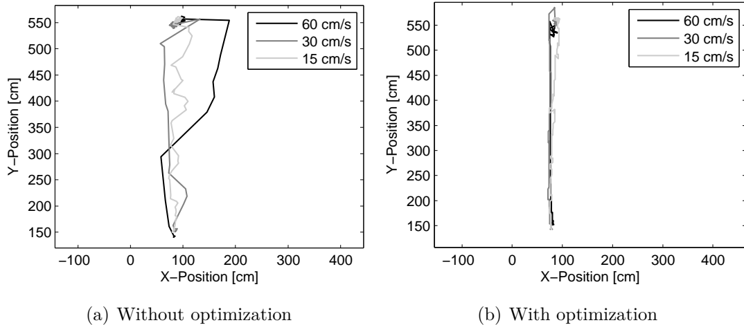
Figure 5.6: Tracking accuracy
