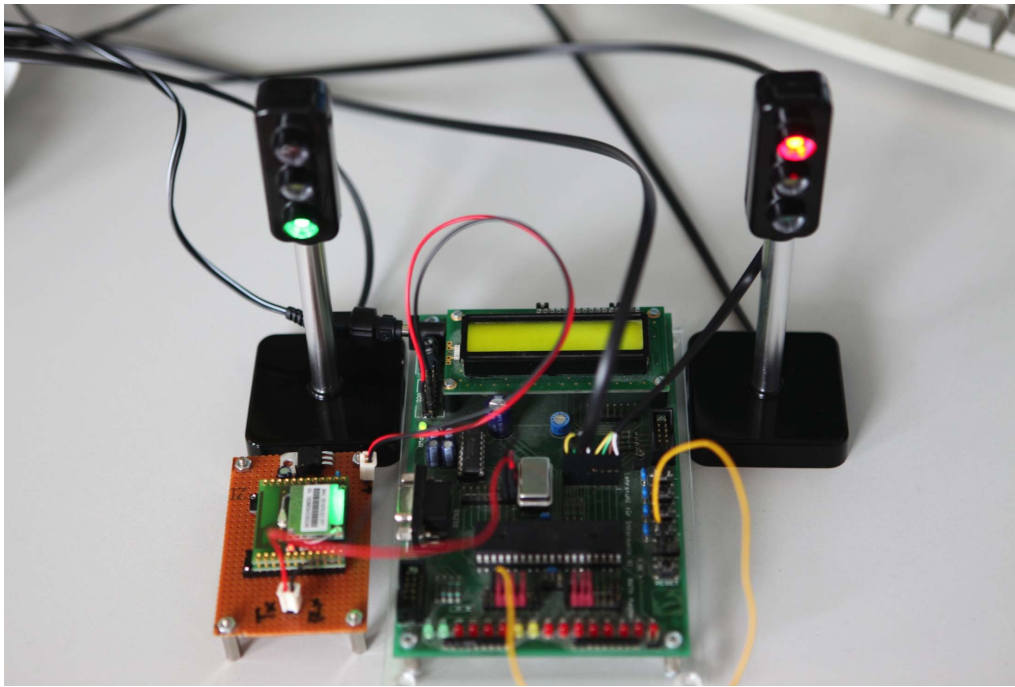
Figure 5.10: Hardware of the traffic light
