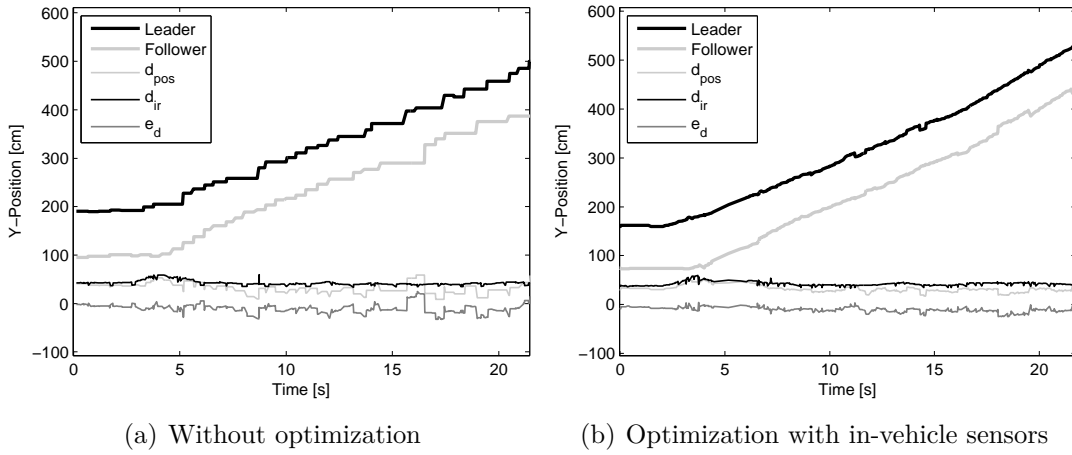
Figure 5.7: Platooning with two trucks and tracking of their y-position
