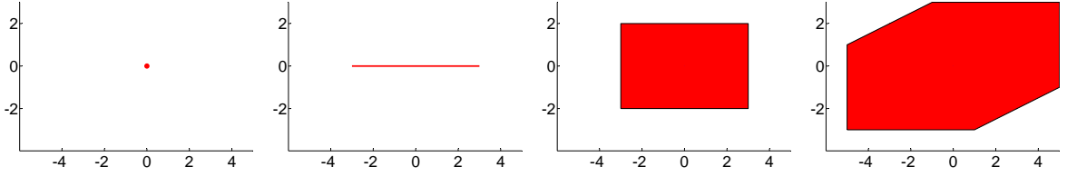
Figure 4.2: Some examples for zonotopes in two-dimensional space
