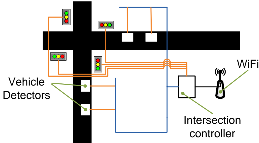
Figure 5.9: Hardware architecture of the intersection management
