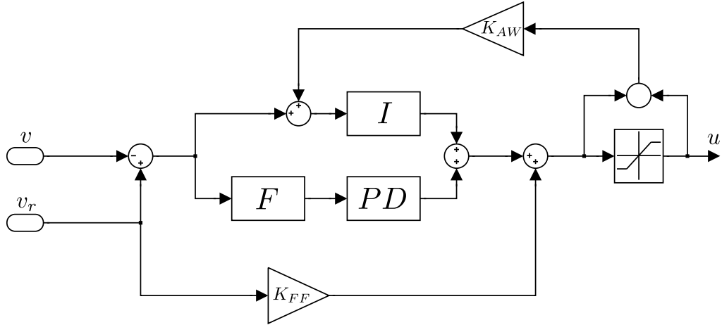
Figure 3.13: Inner loop of the control structure [DCGBM + 10]
