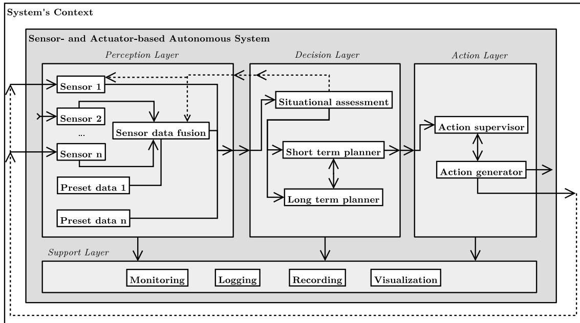
Figure 2.3: General system architecture of a sensor- and actuator-based autonomous system consisting of a Perception Layer , a Decision Layer , and an Action Layer . The leftmost layer is responsible for gathering information from the system's context by processing incoming data from all available sensors. Furthermore, this layer applies algorithms for fusing and optimizing potentially uncertain sensors' raw data to derive a reliable abstract representation. This abstract representation is the input data for the next layer which interprets and evaluates this abstract model to derive an action. This action is passed to the rightmost layer which calculates required set points for the control algorithms. To support the development as well as to supervise the data processing chain which is realized by the aforementioned three stages the support layer provides appropriate tools for visualizing, capturing, and replaying data streams. The overall data processing chain realized by this architecture is closed by the environmental system's context as indicated by the dotted arrows.
