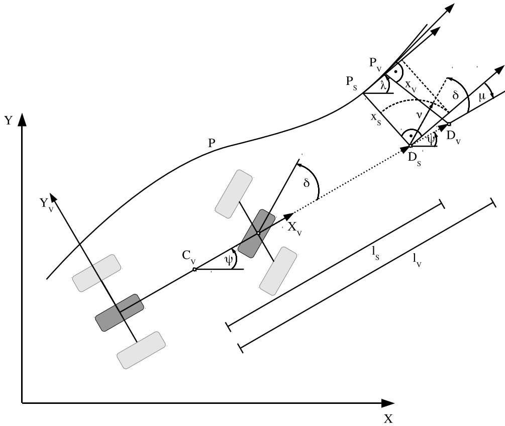
Figure 8.16: Geometrical relations for the control algorithm: The control algorithm based on two independent draw-bars. The first draw-bar called l_s is used for computing the distance x_s to the planned path P , while the latter has a greater distance to the vehicle and is called l_v for computing the distance x_v . The distance x_s is used to steer the vehicle depending on the distance, while the distance x_v is used to adjust the vehicle's velocity by reciprocally proportionally evaluating its value.
