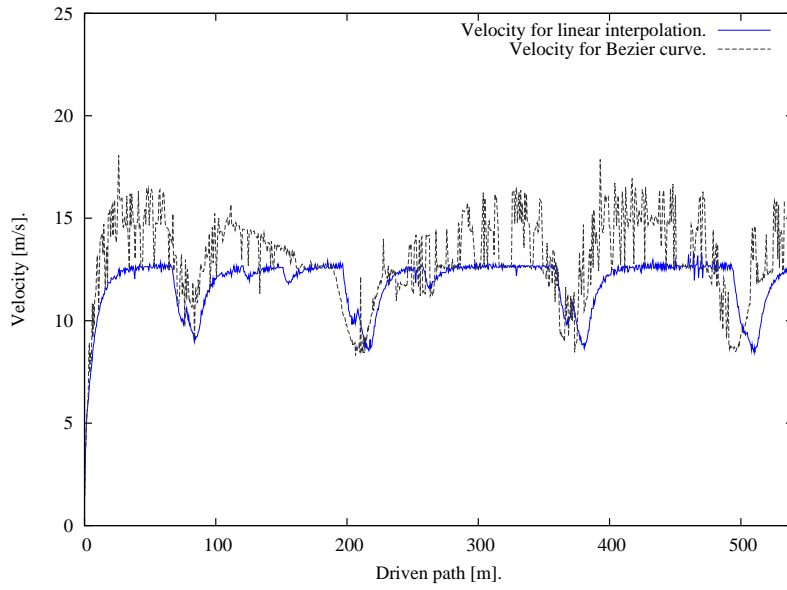
(a) Velocity profile over driven path for linear and B-spline interpolation for v \approx 3.0 \frac{m}{s} .
