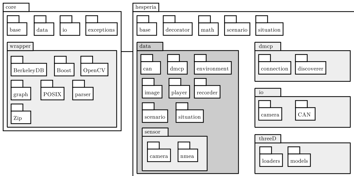
Figure 5.2: Packages of the framework Hesperia : The left hand side is realized in libcore which encapsulates the access to the operating system and to third party libraries as already mentioned. The right hand side is realized in libhesperia . Besides high-level concepts for transparent communication for example, basic data structures which support the development of sensors-based applications which operate in the \mathbb{R}^3 are provided. Furthermore, device-independent visualization concepts which are outlined in Section 5.4.5 are integrated.
