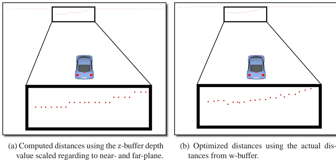
Figure 6.11: Aliasing effect when solely using the z-buffer demonstrated at a curved target: On the left hand side, the rays from the laser scanner are hitting the target with only discrete distances which provides inaccurate distances. This is caused by the decreasing accuracy for increasing distances to the ray-emitting source [32]. On the right hand side, the z-buffer combined with the w-buffer is used to optimize the calculated distances which reduces the aliasing effect.
