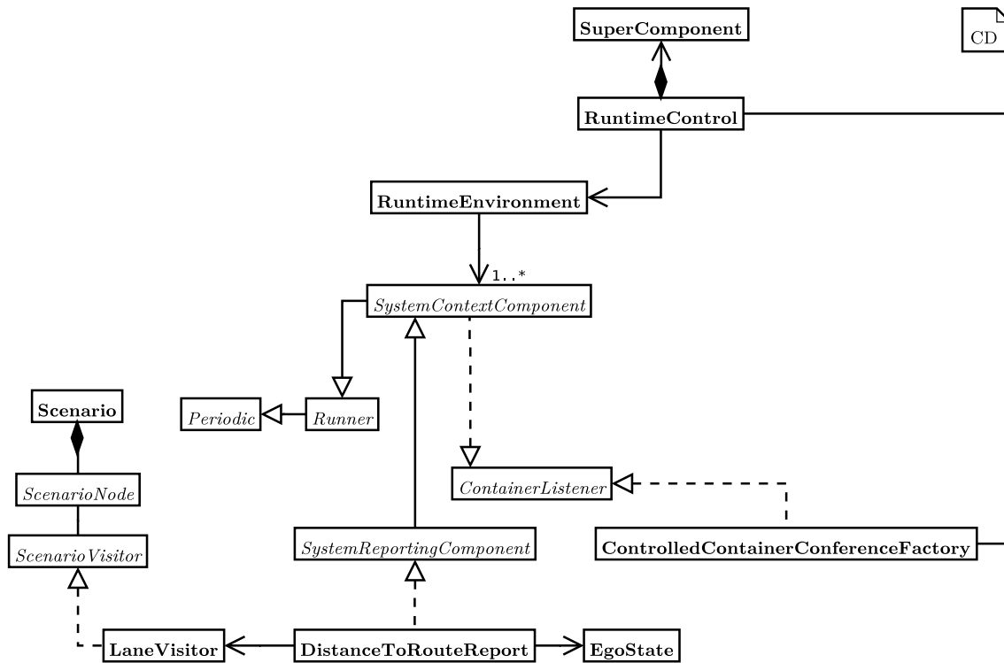
Figure 7.8: Software architecture for a SystemReportingComponent to evaluate whether the vehicle’s distance to an optimal route is continuously less than a given threshold. Therefore, comparable to the aforementioned component, DistanceToRouteReport automatically receives all distributed Containers and evaluates the current vehicle’s position and orientation to a pre-calculated given or to the optimal route using a LaneVisitor which traverses the road network.
