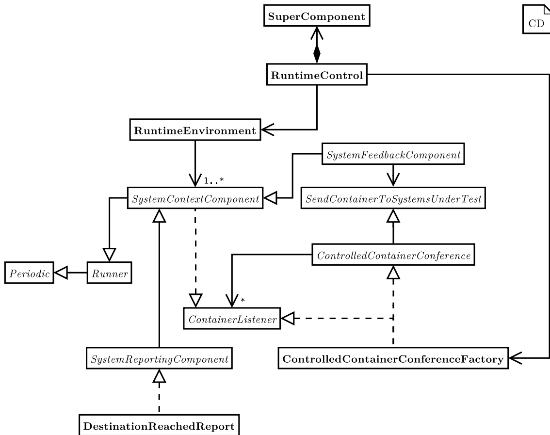
Figure 7.6: Software architecture for reporting components which evaluate the system's context. All reporting components derive from SystemReportingComponent which allows a specified frequent scheduling by RuntimeControl . Furthermore, these components are automatically receiving all sent Containers for evaluation.
