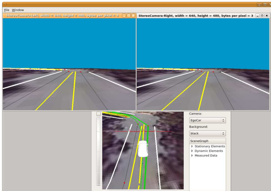
Figure 8.15: Non-reactive visualization of the Ford Escape Hybrid – ByWire XGV’s sensors’ model: In the upper area both raw images from the stereo vision system are shown. Below these images, the chasing camera for the AGV which is indicated by the white vehicle is shown. This camera is continuously following the vehicle’s movements and thus, from this perspective, the scan line for the single layer laser scanner can be seen in front the car.
