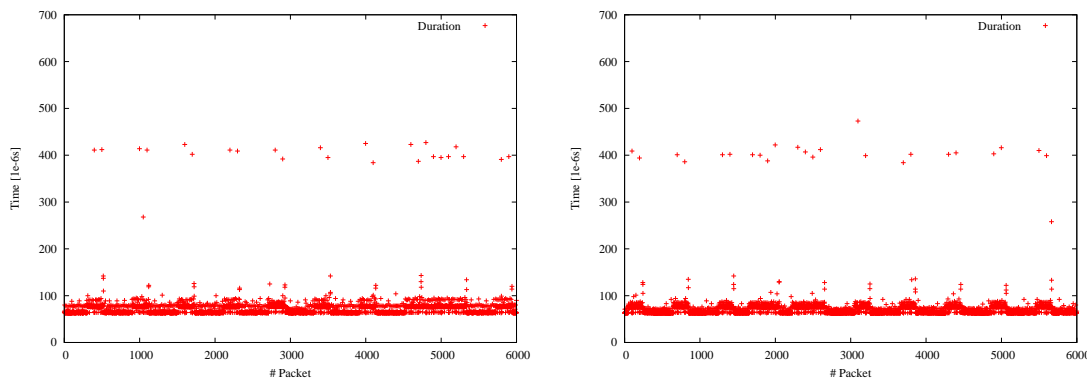
(a) Benchmark for one sender sending data at 100Hz and one receiver running as user processes on the same computer. (b) Benchmark for one sender sending data at 100Hz and one receiver running as privileged processes on the same computer.
