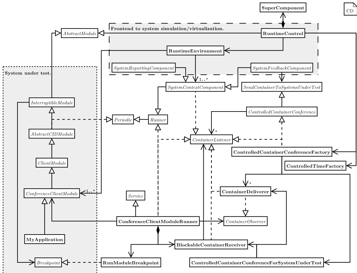
Figure 6.3: Run-time control for the SUD: On the left hand side, the SUD is shown which implements automatically the interface InterruptibleModule and Periodic . While the former is required to register a special object called Breakpoint to intercept regularly the running application, the latter is necessary to calculate and realize a system-wide scheduling which is implemented by RuntimeEnvironment . This class controls and schedules the required components' frequencies; furthermore, it supervises the sending and receiving of Containers by using the class ControlledContainerConferenceFactory .
