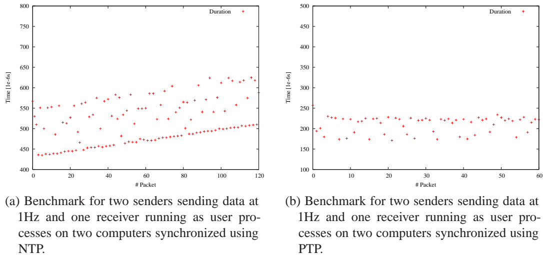
Figure 8.9: Comparison between NTP and PTP: The plot on the left hand side is translated to the bottom to allow a more intuitional comparison because the measured durations on the left hand side have an additional offset. However, this inaccuracy is within the NTP's specification which is under ideal conditions at least a multiple of 1 \times 10^{-6} s according to [103].
