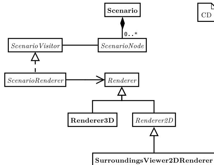
Figure 5.6: Device-independent data visualization: Any data which should be visualized uses the interface Renderer which provides rudimentary drawing primitives for drawing points or lines in \mathbb{R}^3 for example. This interface is implemented by a concrete implementation for the OpenGL context which is also provided by libhesperia . For generating a 2D view on a given data, some methods from the interface Renderer are combined by flattening the z coordinates which is realized in the abstract class Renderer2D . Thus, a concrete realization which uses this class simply implements the reduced set of drawing primitives which is outlined in Section 7.2.
