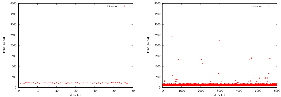
(a) Benchmark for two senders sending data at 1Hz and one receiver running as user processes on two computers synchronized using PTP: The average transmission duration is at approximately 0.209ms while the worst case transmission duration is at 0.429ms.
