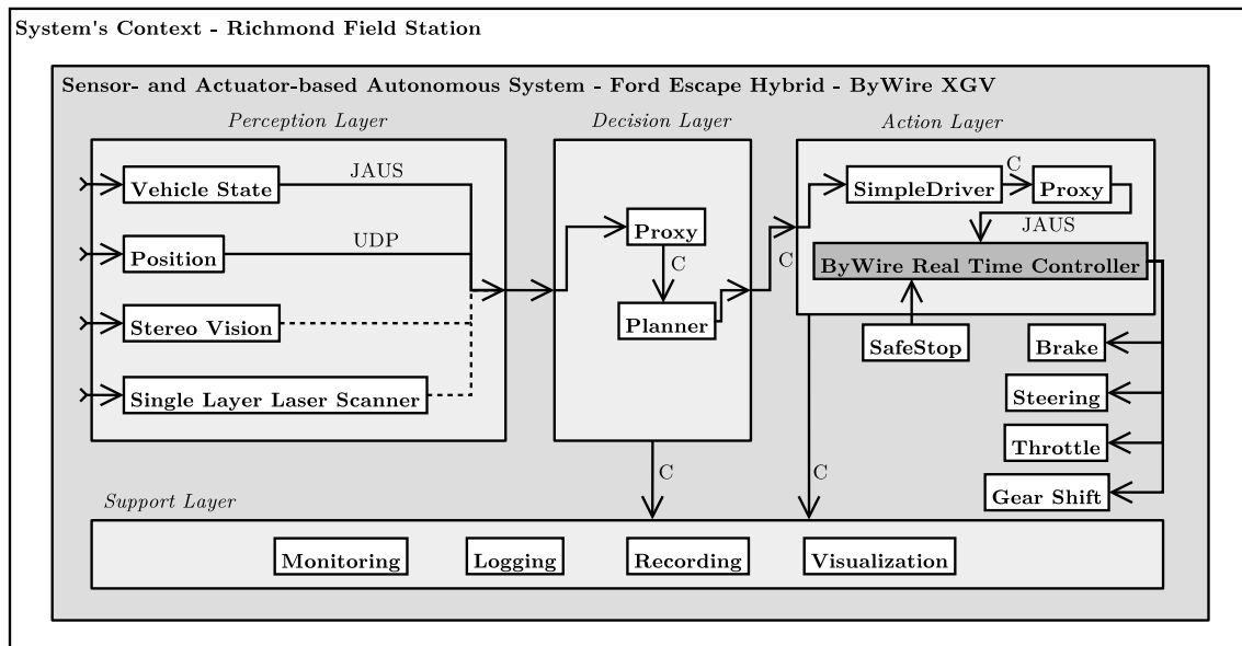
Figure 8.11: System architecture implemented in the 2008 Ford Escape Hybrid – By-Wire XGV. JAUS indicates data which is encapsulated into the JAUS protocol, UDP indicates data which is sent using a proprietary protocol, and C indicates data wrapped into a Container data structure; therefore, the application proxy from the framework Hesperia is used. Furthermore, the components Planner and SimpleDriver are realized as one combined application using the framework Hesperia as well. The applications from the support layer are described in Section 5.5, 5.6, and 7.2 and base also on the framework Hesperia .
