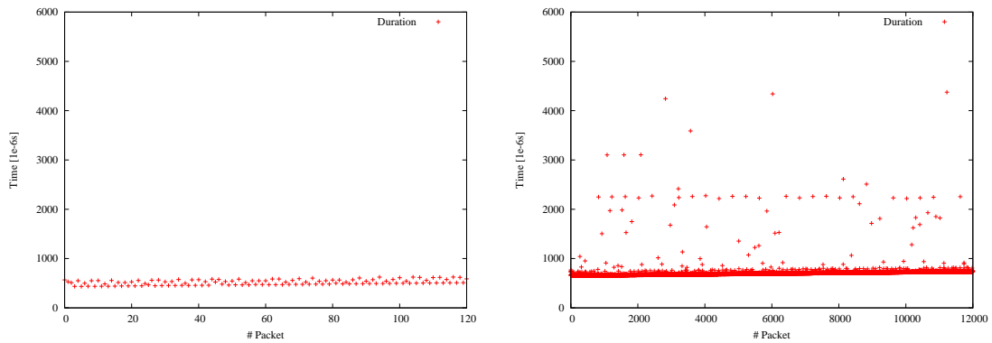
(a) Benchmark for two senders sending data at 1Hz and one receiver running as user processes on two computers synchronized using NTP: The average transmission duration is at approximately 0.591ms while the worst case transmission duration is around 0.768ms.
