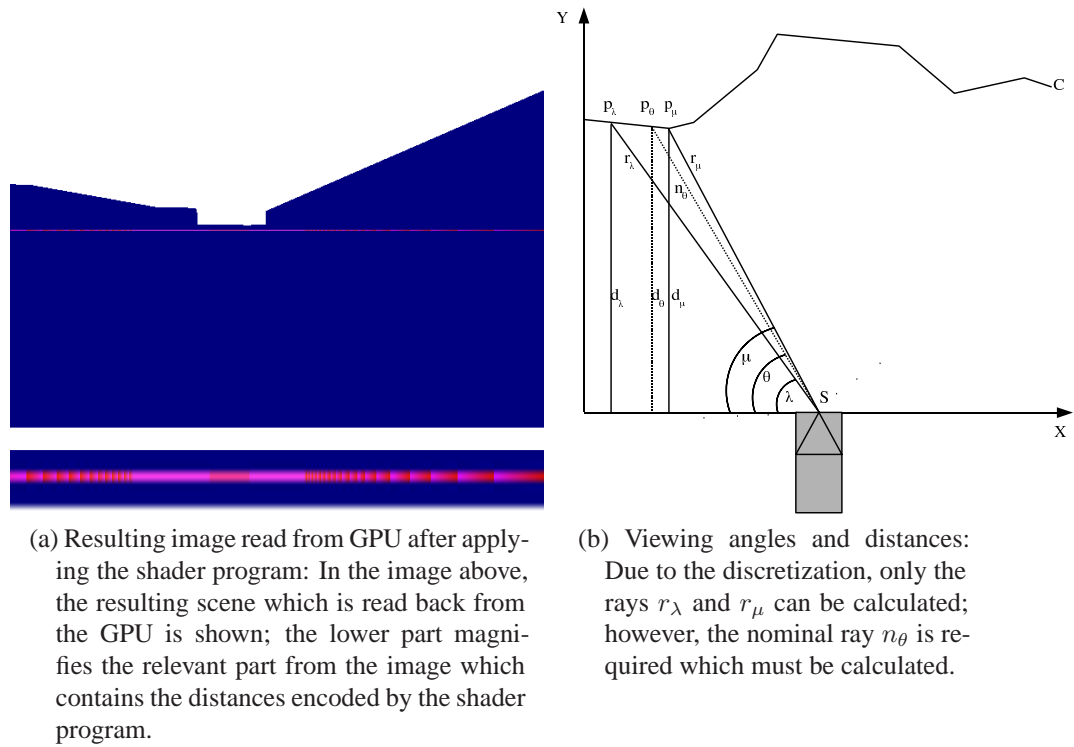
Figure 6.10: Visualization for the output of the sensor model for a single layer laser scanner. This sensor model is realized in an application which uses a shader program on the GPU for calculating the distances.
