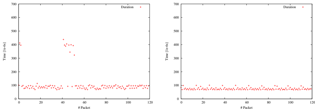
(a) Benchmark for two senders sending data at 1Hz and one receiver running as user processes on the same computer: The average duration is around 0.126ms with a worst case duration at approximately 0.438ms.
