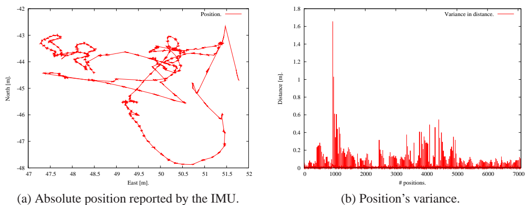
Figure 8.13: AGV's absolute position provided by the IMU over time and its variance.
