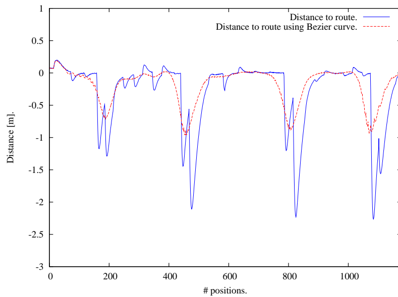
(b) Linear distance to planned path for v \approx 2.3 \frac{m}{s} .
