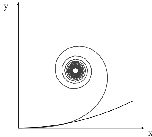
Figure 4.5: Fresnel integral together with an approximation using a 3rd order polynomial with d_\kappa = 0.0215 and \kappa = 0.215 which are estimated values to approximate the beginning of the Fresnel integral. For road segments which shall be modeled with a 3rd order polynomial instead of clothoids, a segment-wise approximation using several 3rd order polynomials with different lengths and coefficients are necessary. An algorithm for a segment-wise approximation of the Fresnel integrals is presented in [111].
