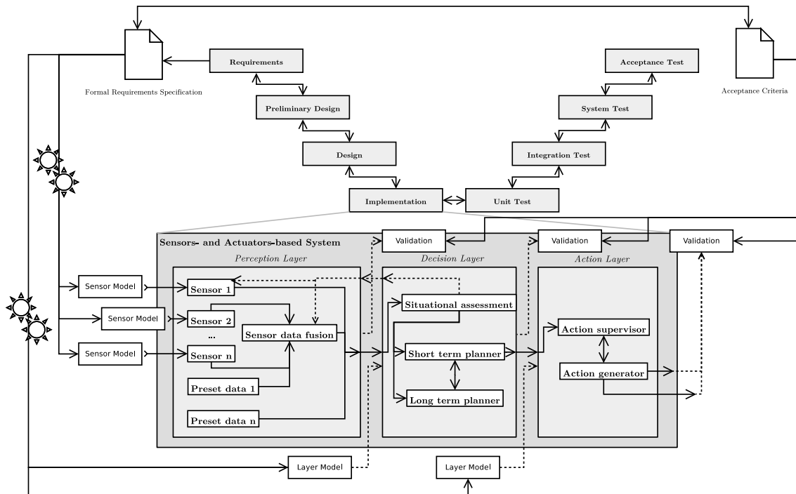
Figure 3.1: Methodology which uses the customer's requirements from the topmost level of the V-model as the basis for a formal specification of the system's context. This specification is used to generate the required input data for the different layers of a sensor- and actuator-based autonomous system. Moreover, completing the customer's requirements, its acceptance criteria are used to specify metrics for evaluating individual layers or the entire data processing system.
