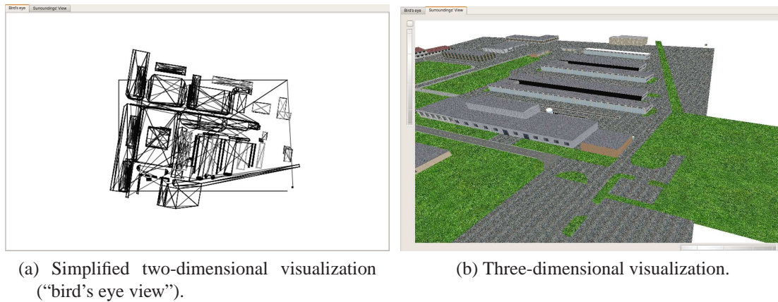
Figure 7.4: Resulting representation using the concept of device-independent visualization. The camera on the right hand side is located in the lower left corner of the two-dimensional image pointing to its upper right corner.
