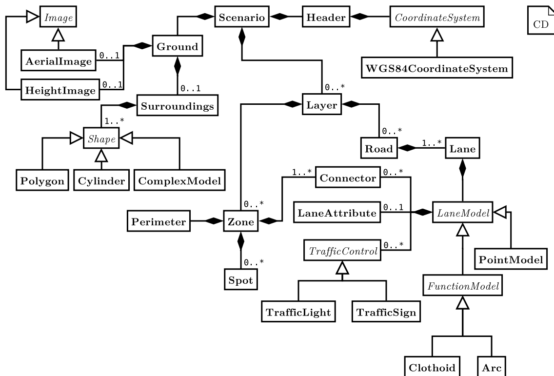
Figure 4.4: UML class diagram describing the system's context's stationary elements. For the sake of clarity only multiplicities other than 1 are denoted. The complete DSL which is derived from this UML class diagram including all attributes can be found in Section A.
