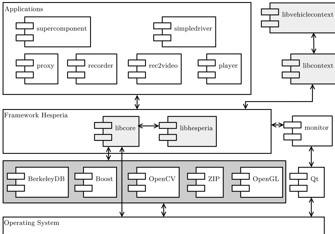
Figure 5.1: Package structure of the framework Hesperia . The framework consists of two major libraries: libcore and libhesperia . The former library encapsulates the interfaces for a specific operating system by providing elaborated programming concepts for I/O access or threading. Furthermore, this library wraps libraries from third parties and provides interfaces instead to higher layers. Thus, a third party library can be easily exchanged if necessary. The latter library, libhesperia provides concepts which allow a simplified development for distributed data processing applications. Therefore, this library provides classes which transparently realize data exchange; moreover, this library contains the DSL which was specified in Section 4.4.
