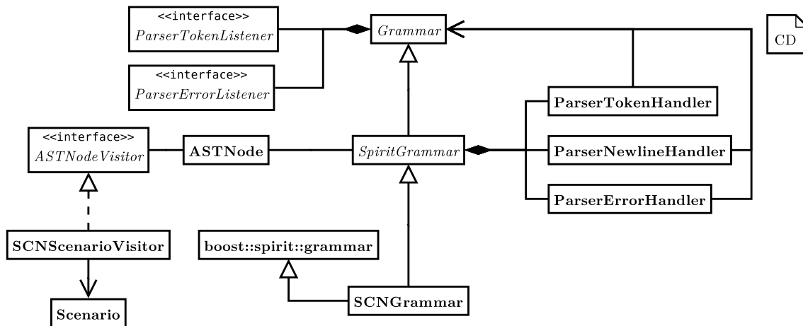
Figure 4.7: Class diagram describing the language processing for the stationary surroundings using Spirit. For the sake of clarity, all methods and attributes are omitted. An implementation-independent interface is realized in the abstract class Grammar . This class provides an observer for successfully parsed token from the grammar which calls a user-supplied listener; analogously realized is an observer which reports parsing errors. These observers are used to construct an AST from a given instance according to the grammar's structure. This AST can be easily traversed by user-supplied visitors to query information from a given instance or to transform the data structure.
