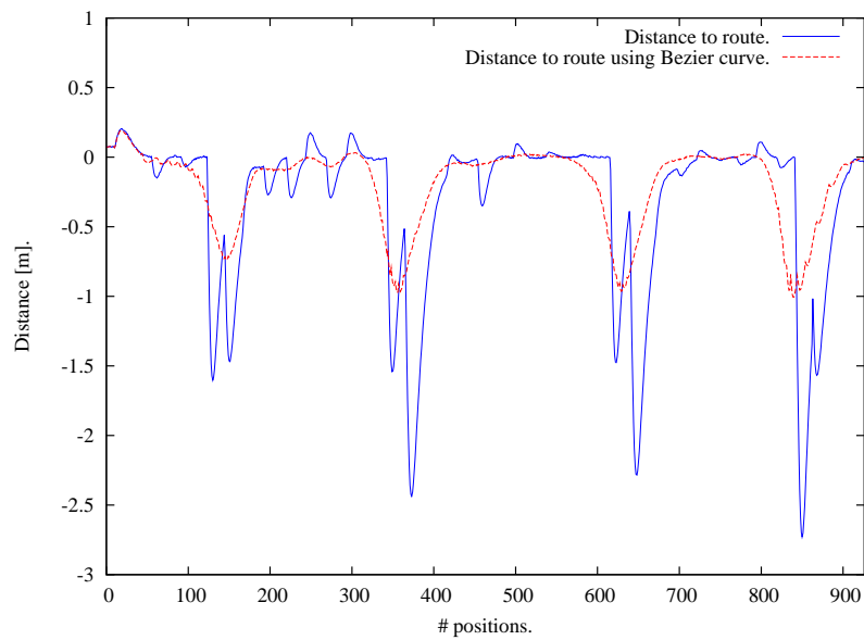
(b) Linear distance to planned path for v \approx 3.0 \frac{m}{s} .
