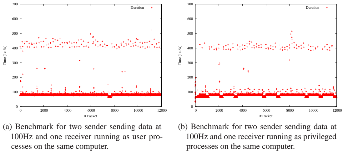
Figure 8.6: Benchmark for two senders sending data at 100Hz and one receiver running on one computer: On higher network traffic on the local network device, no significant difference between privileged and non-privileged processes can be deduced.
