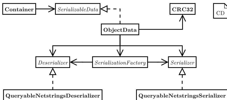
Figure 5.4: Template-based query-able serialization: The data to be serialized is realized by ObjectData . This class derives from the interface SerializableData which itself provides serialization and deserialization methods which are called by the envelope data structure Container . These methods are realized using the supporting classes Serializer and Deserializer which encapsulate the handling of hardware-dependent endianness for example.
