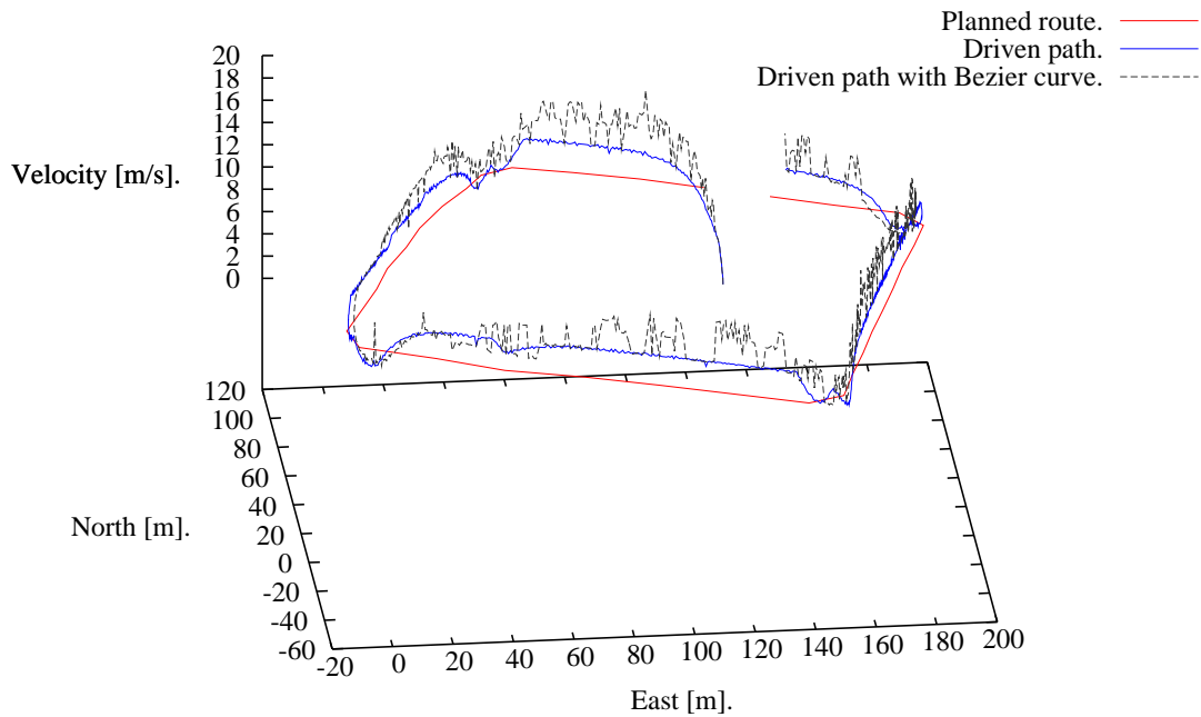
(b) Velocity relative to planned route for linear and B-spline interpolation for v \approx 3.0 \frac{m}{s} .
