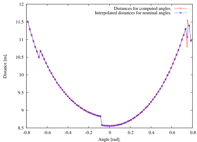
(b) Plot of interpolated distances for nominal angles and computed angles for measured distances: The graph marked with + shows the computed angles while the graph marked with x depicts the reconstructed nominal angles.
