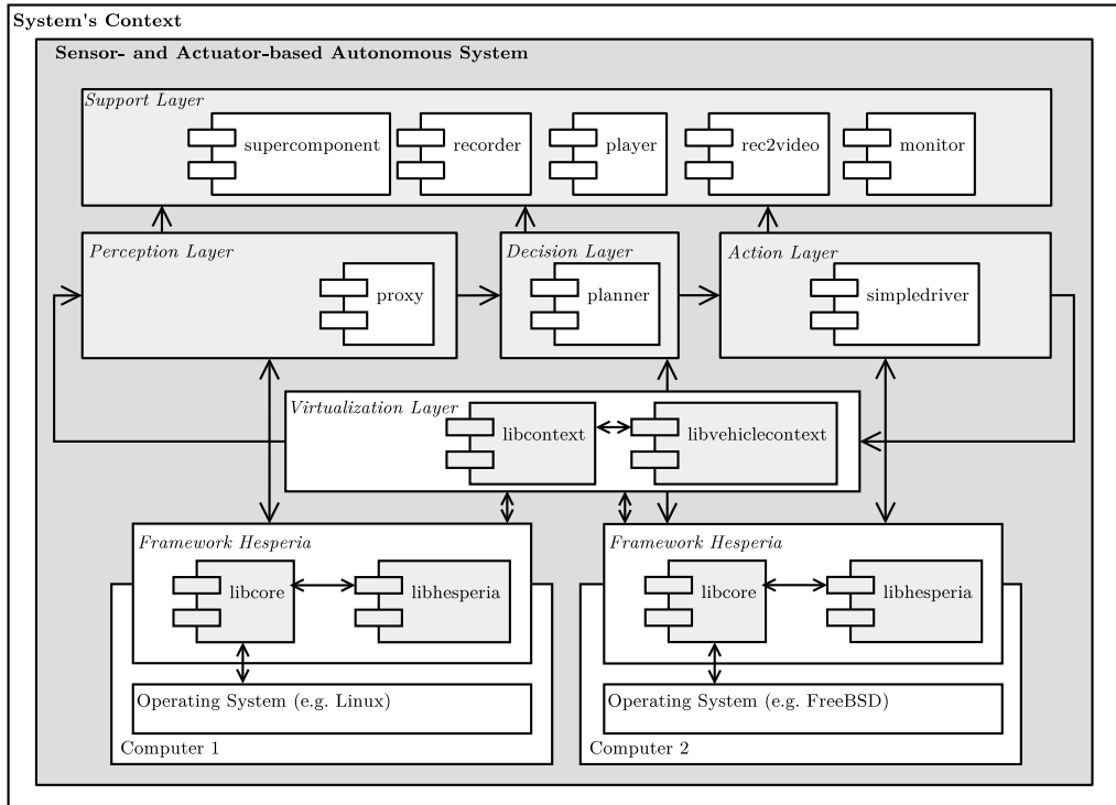
Figure 6.1: Integration of the system simulation within the framework Hesperia : Using concepts and algorithms from Hesperia , the application which realizes the sensor- and actuator-based system is on top of Hesperia . For closing the loop between the action layer and the perception layer to enable interactive and unattended simulations, the virtualization layer with libcontext and libvehiclecontext is used. While the former is necessary to realize the run-time discretization for the SUD by providing time control and scheduling, the latter provides models like the bicycle model for the specific use for autonomous vehicles for example. Thus, the framework Hesperia provides an application-independent virtualization layer to realize system simulations.
