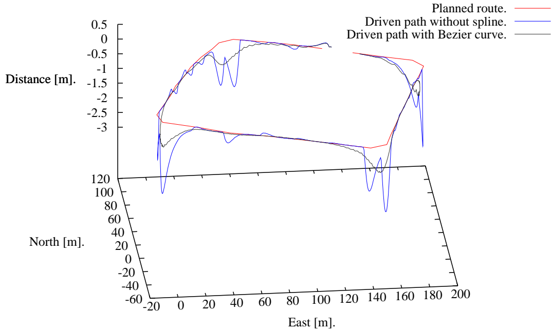
(a) Planned route with driven path for v \approx 3.0 \frac{m}{s} .
