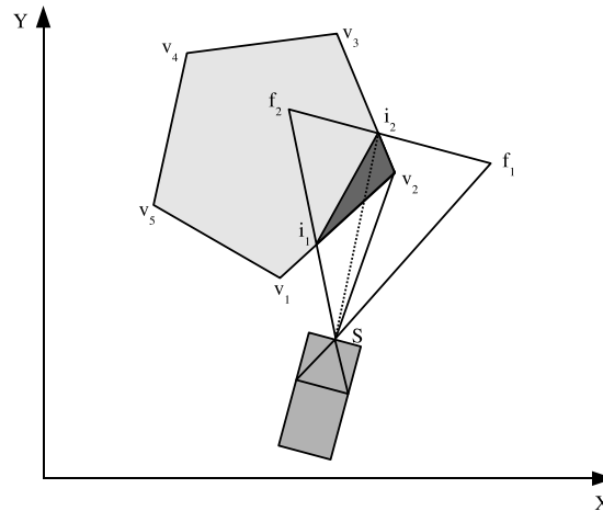
Figure 6.14: Overlapping polygons with visibility lines resulting in a contour line between i_1 and v_2 : The dark gray triangle i_1, v_2, i_2 shows the invisible area within the sensor's FOV from point S for the polygon v_1, v_2, v_3, v_4, v_5 . Because the line \overline{Si_2} crosses this invisible area, the point i_2 is not part of the outer contour.
