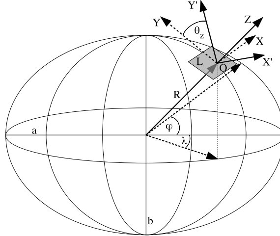
Figure 4.2: Cartesian coordinate system based on WGS84 origin. a denotes the the equatorial diameter, b denotes the North/South diameter. The triple (R, \varphi, \lambda) which consists of the radius and a spherical coordinate in WGS84 denotes a coordinate on the Earth's surface pointing to the origin O of a Cartesian coordinate system L . The normal vector for this coordinate system is described by the aforementioned triple.
