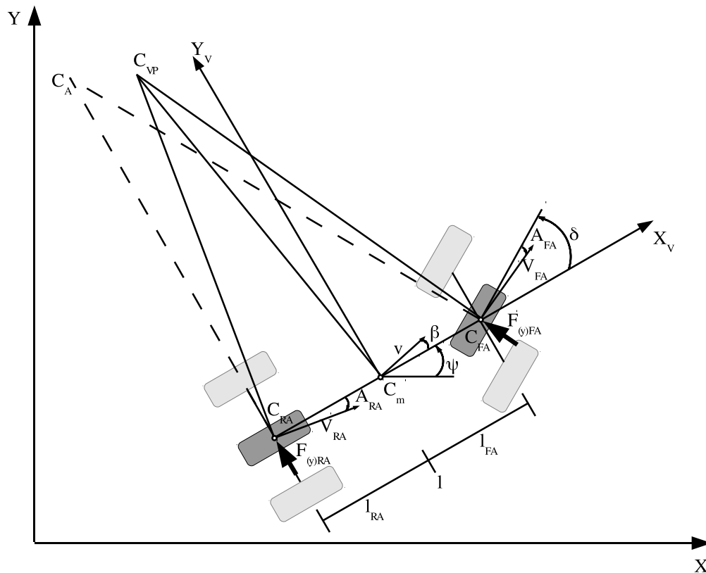
Figure 6.5: Geometry of the bicycle model (based on [126]).
