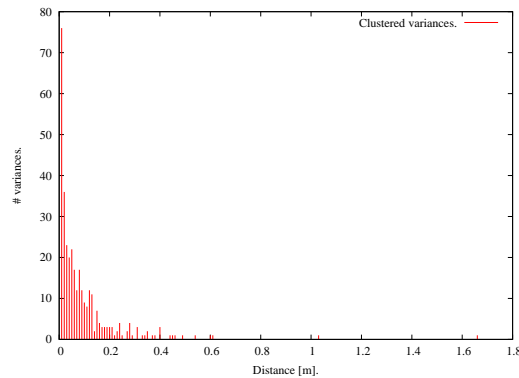
Figure 8.14: Clustered variances for the IMU provided positions.
