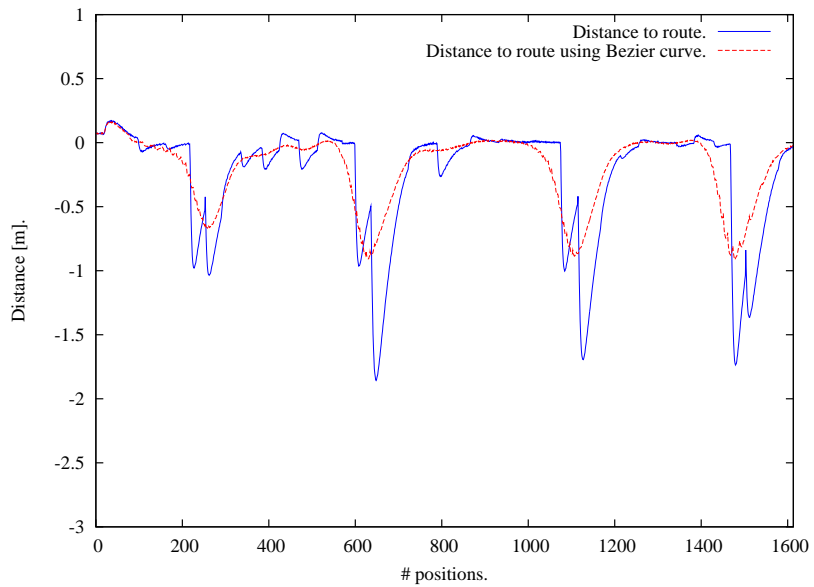
(b) Linear distance to planned path for v \approx 1.6 \frac{m}{s} .
