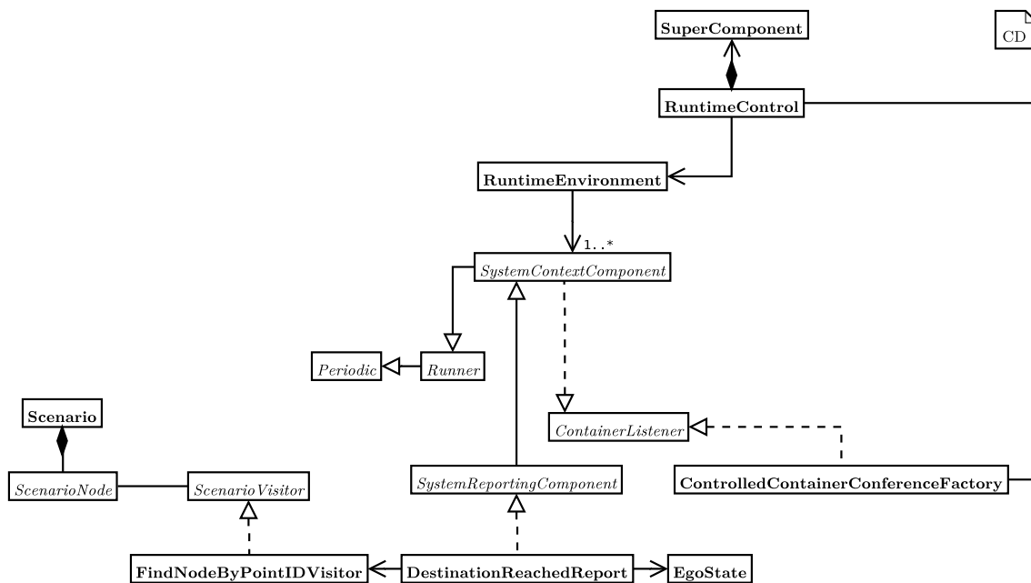
Figure 7.7: Software architecture for reporting whether a given destination was successfully reached. The DestinationReachedReporter implements the interface SystemReportingComponent to receive automatically all send Containers. Furthermore, it uses the formally specified scenario for getting information about available way-points which can be used as destinations for an AGV.
