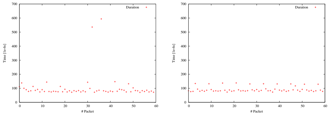
(a) Benchmark for one sender sending data at 1Hz and one receiver running as user processes on the same computer: Some packets are delayed up to 0.6ms. (b) Benchmark for one sender sending data at 1Hz and one receiver running as privileged processes on the same computer: When the same test is carried out using a privileged user the average duration is approximately at 0.0936ms without the aforementioned peaks.
