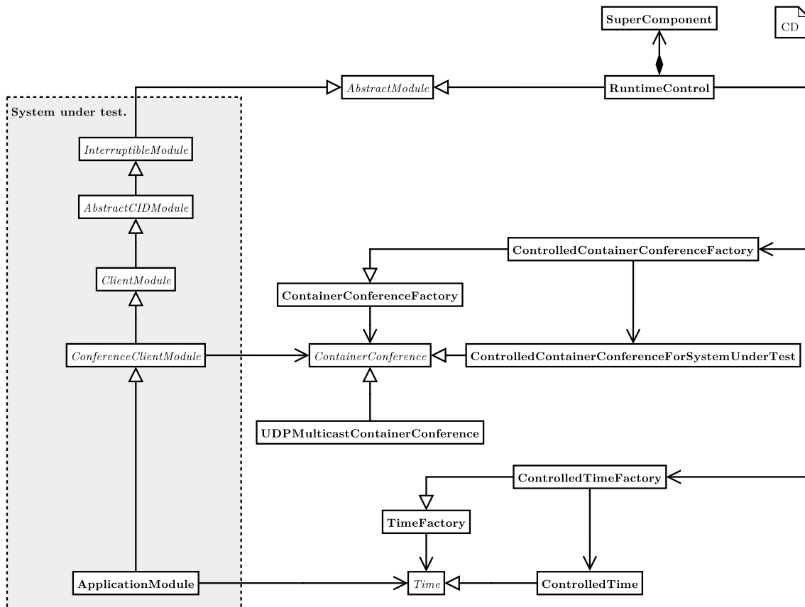
Figure 6.2: Control of time and communication: On the left hand side, the SUD is shown which is realized in ApplicationModule by the user. For controlling the overall system time and communication, the class RuntimeControl overrides the regular implementation of ContainerConferenceFactory by providing a pure software solution which manages the sending and receiving of Containers between several applications. The same concept is applied to the TimeFactory which is intercepted by a specialized variant which allows the controlled incrementation of the system-wide time.
