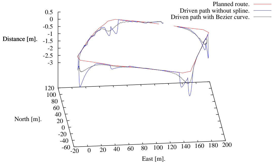
(a) Planned route with driven path for v \approx 1.6 \frac{m}{s} .
