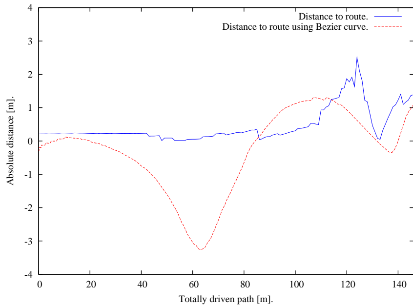
(b) Linear distance relative to the planned route for the velocity and steering control algorithm in reality for v \approx 4.1 \frac{m}{s} .
