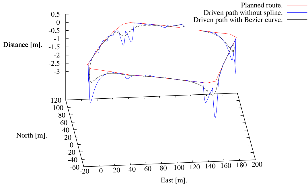
(a) Planned route with driven path for v \approx 2.3 \frac{m}{s} .
