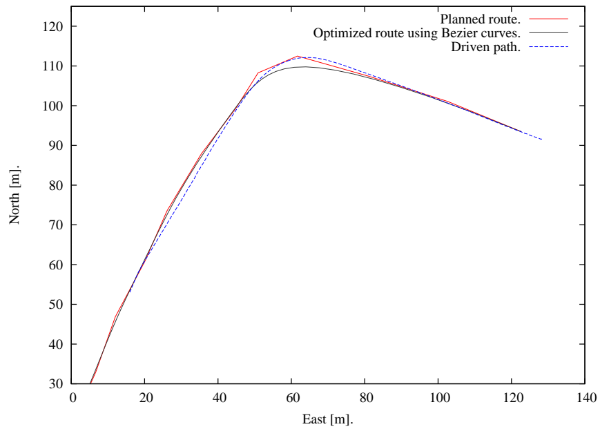
(a) Performance of the velocity and steering control algorithm in reality for v \approx 4.1 \frac{m}{s} : The red line interconnects the single way-points of the road network and the black line depicts the optimized route using a Bézier curve. The finally driven blue line is the actual position of the AGV in reality.
