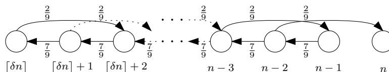
Fig. 2: Transition probabilities of the random walk.
