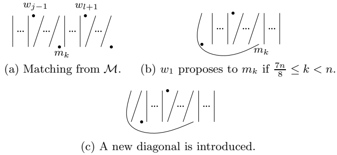
Fig. 4: One phase of the best response dynamics.
