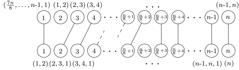
Fig. 3: Nodes in the upper and lower row correspond to women and men respectively. The figure also shows the initial state and the preference lists. The lists are only partially defined, but they can be completed arbitrarily.
